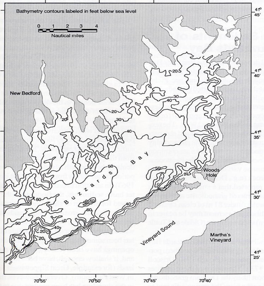
Fig. 2.4. Bathymetric contours of Buzzards Bay adjusted to mean low water datum. From Moore (1963).
